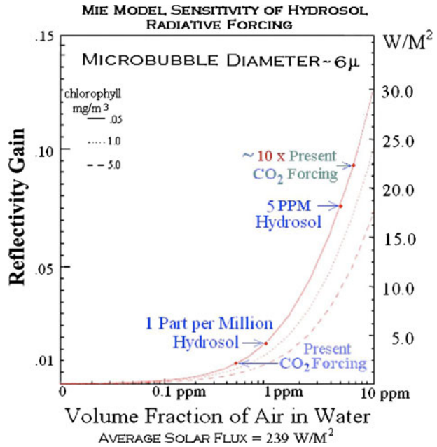
Fig. 3 Mie model results (see Jin et al. 2006 for model details) indicating the increase in the reflectivity gain (i.e., albedo increase) that can be achieved as a result of increasing the volume fraction of air in water using 6- \mu\text{m} bubble diameter. Results are shown for differing amounts of chlorophyll in the water, and for various \text{CO}_2 forcing levels
