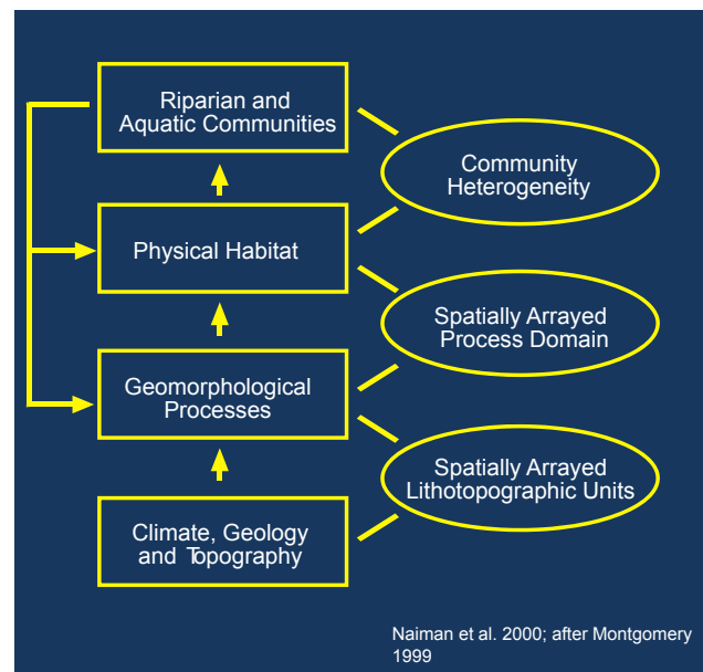
Fig. 2. Schematic representation of the relations among hydrogeomorphic processes, habitat dynamics, and riverine communities. Lithotopographic units are areas with similar topography and geology, and within which similar suites of geomorphic processes occur (Naiman et al. 2000; modified from Montgomery 1999).
