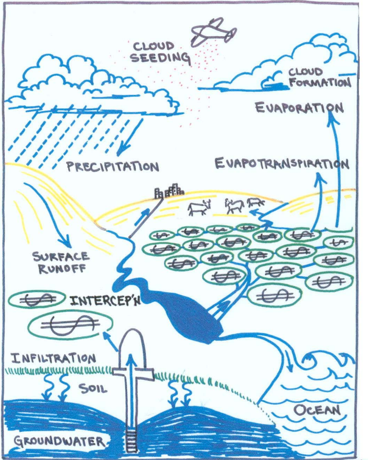
The hydrologic cycle as it occurs today. Water flows to money!
