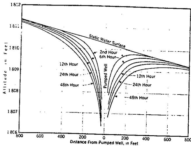
FIG. 2. GROWTH OF CONE OF DEPRESSION DURING PUMPING TEST IN PLATTE VALLEY, NEBR.
